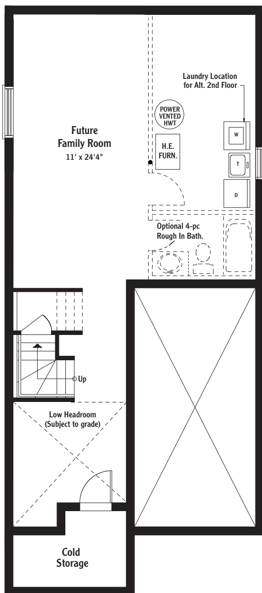
Basement Plan
