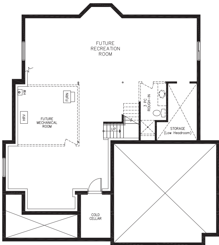
Basement Plan Not to scale
